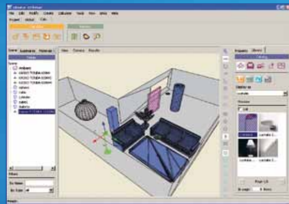
Lighting design for interiors
